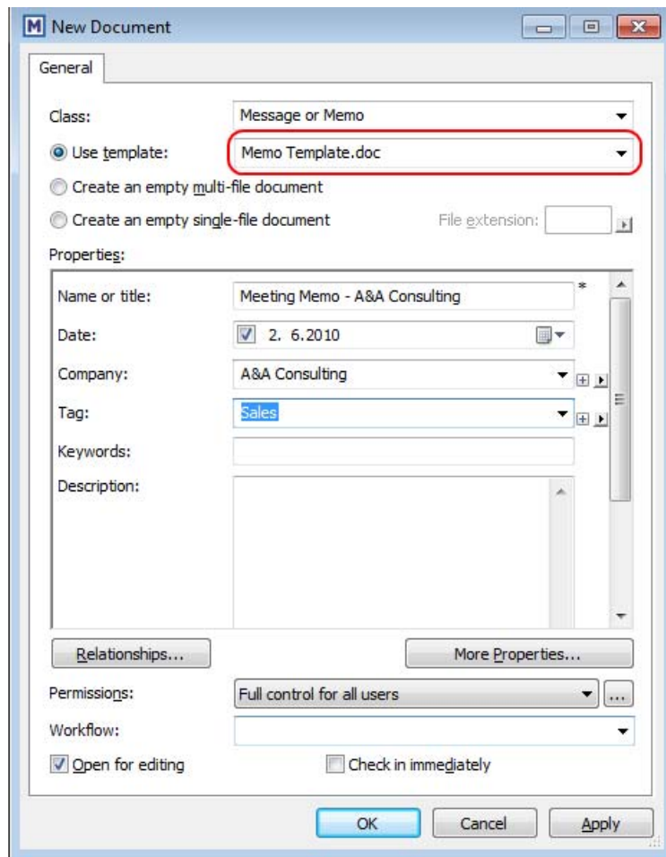
Figure 6 - Create document using a template
