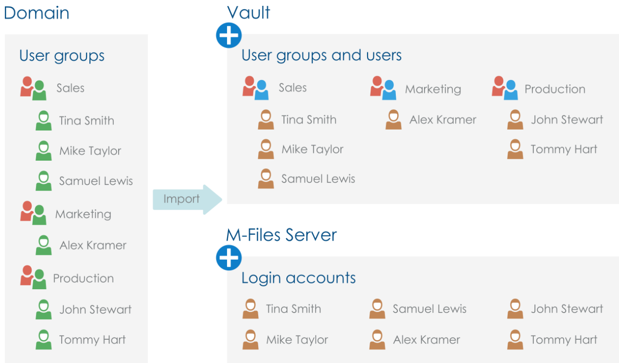
Figure 48: User groups can be imported from the domain to the vault, allowing existing user groups in the domain to be used for specifying permissions to vault content.
