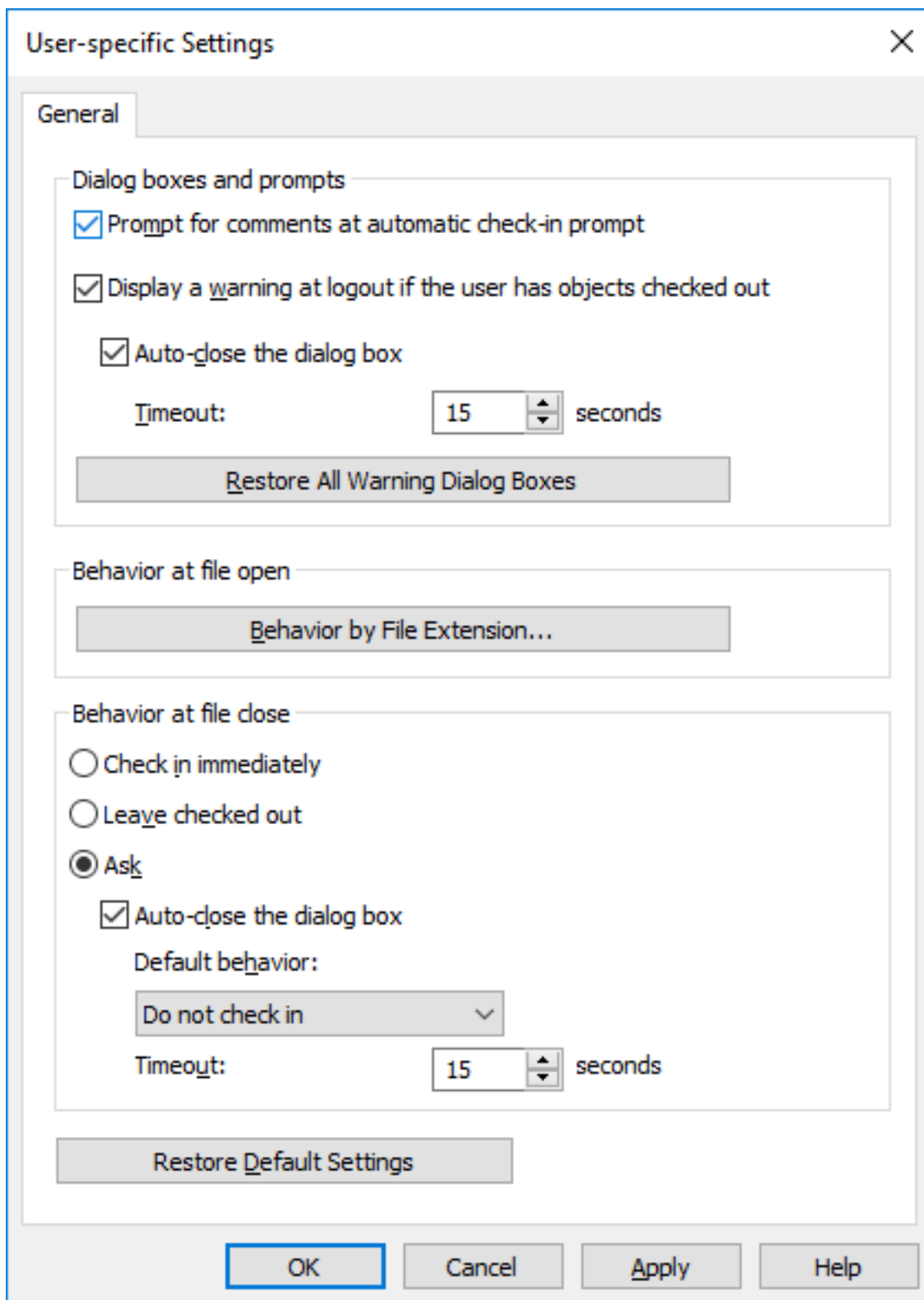
Figure 11: The user-specific settings are specific to Windows users per workstation.
