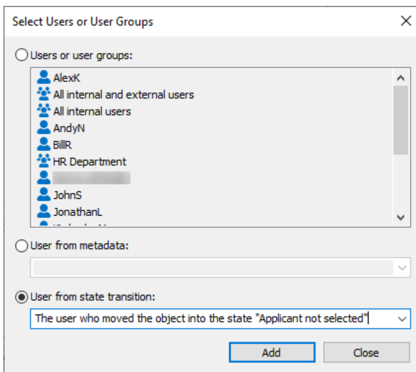
Figure 56: Selecting a user based on an earlier state transition.
