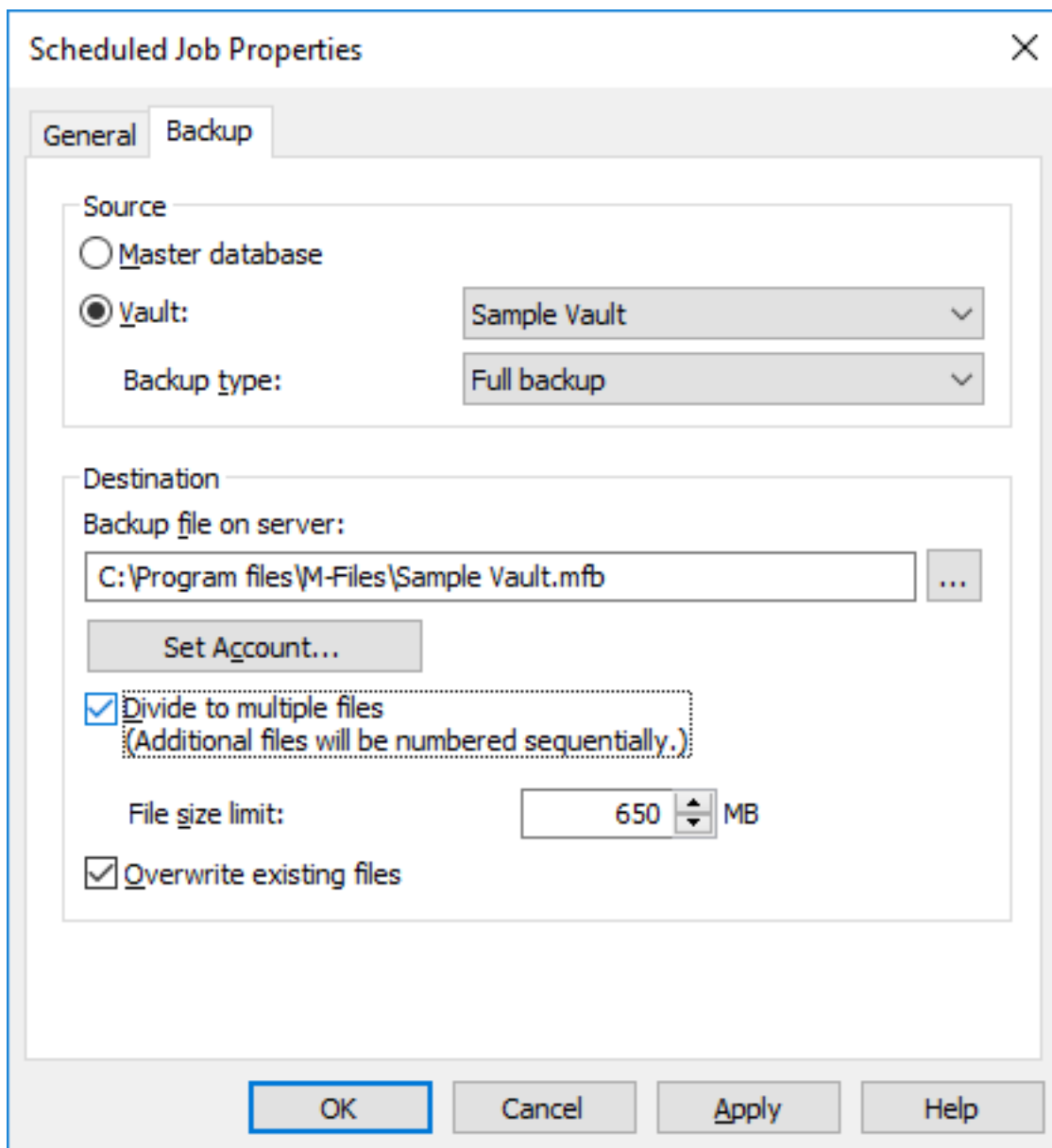
Figure 26: The Backup tab of the Scheduled Job Properties dialog.
