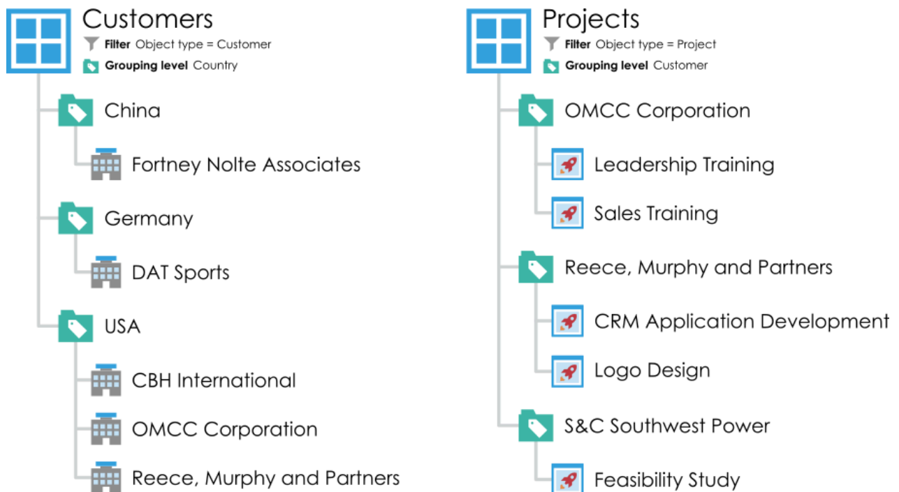
Figure 8: These examples use customer, project, and country information to group objects.
