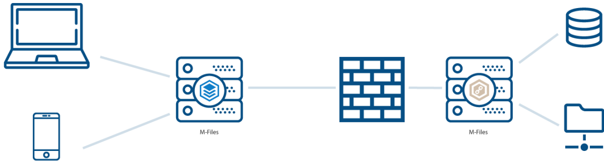
Figure 68: A Ground Link proxy lets a vault connect to private repositories, such as network folders, without a direct network path.
