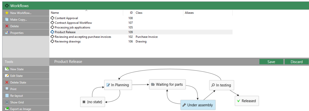
Figure 52: The graphical workflow designer in M-Files Admin.
