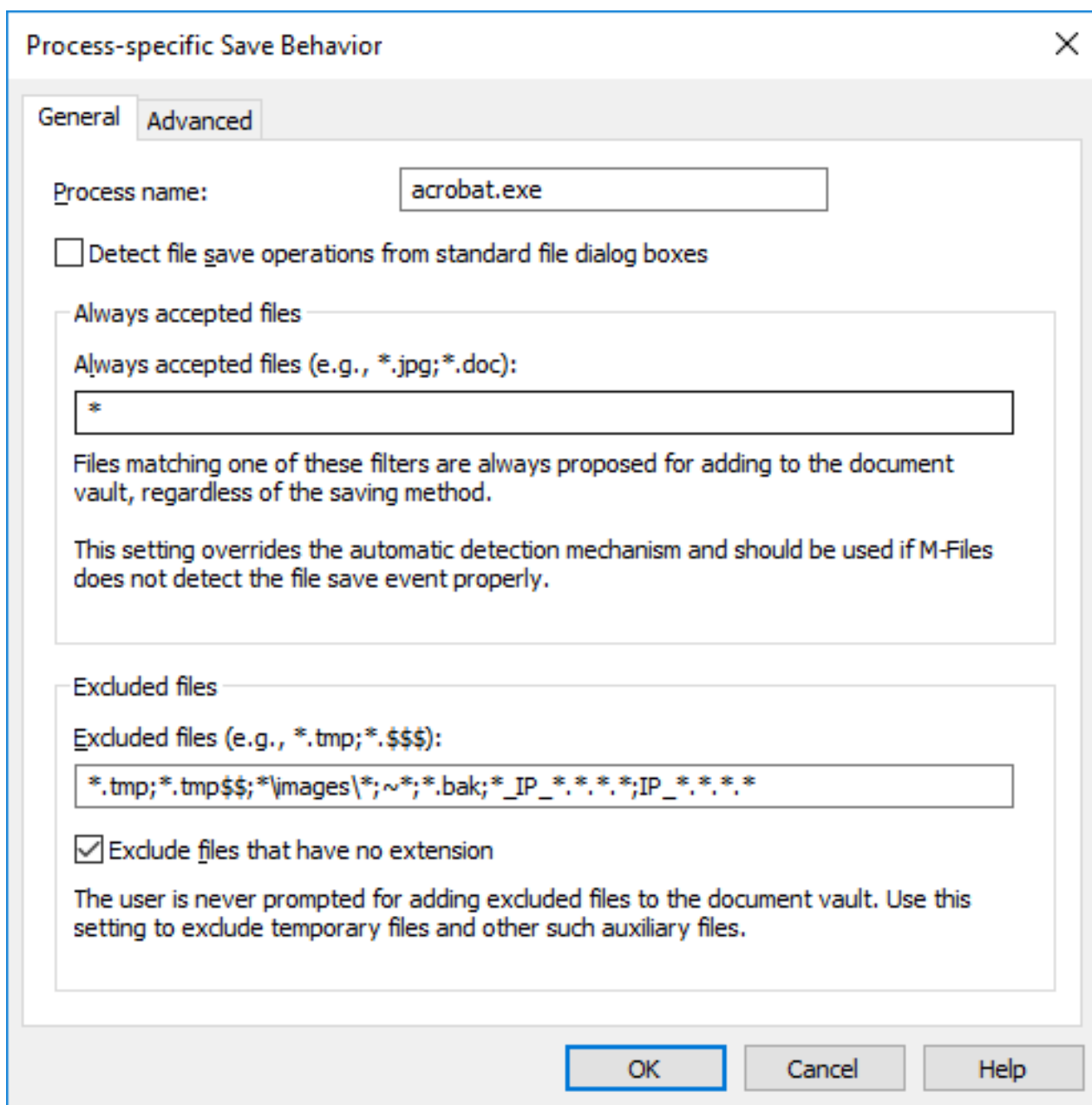
Figure 15: General process-specific settings.
