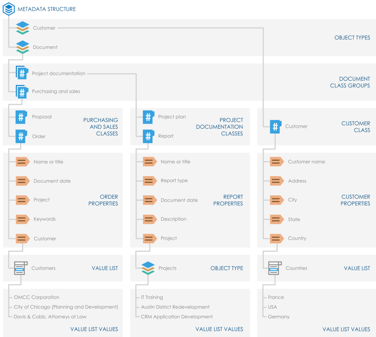
Figure 39: The vault metadata structure consists of object types, class groups, classes, property definitions, and value lists. The example above illustrates the hierarchy of a metadata structure that contains the Customer and Document object types and various classes for the two object types.
