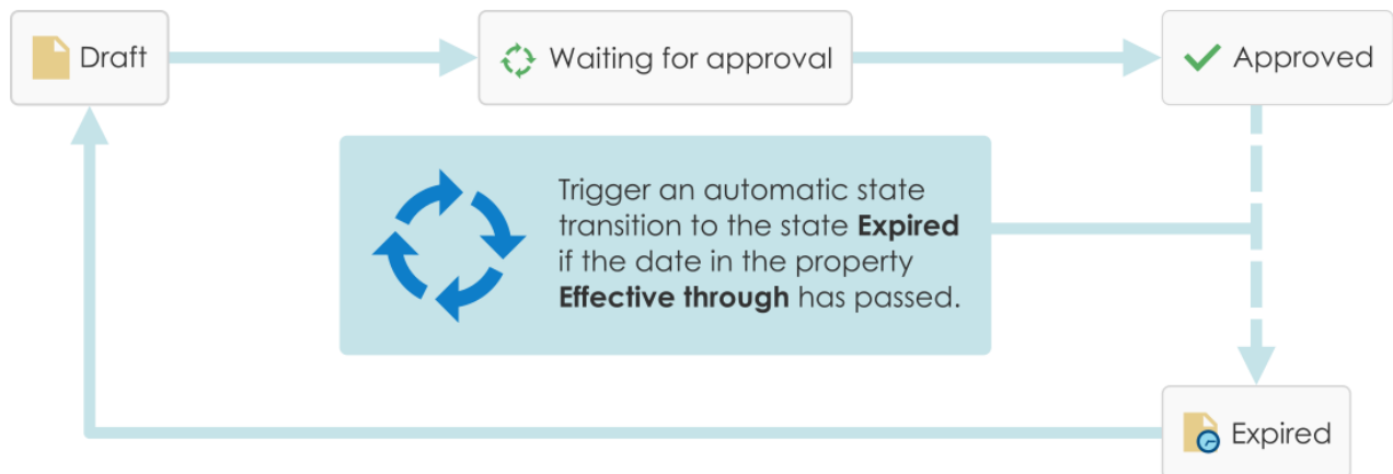
Figure 63: An automatic state transition for an object can occur for example on the basis of the property values of the object.
