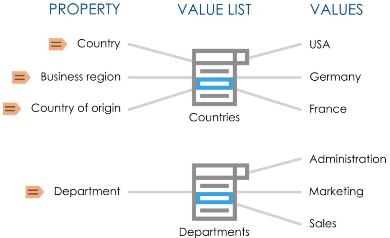
Figure 40: Value lists can be used for storing and selecting preset values for metadata properties. Several different properties can be based on the same value list.
