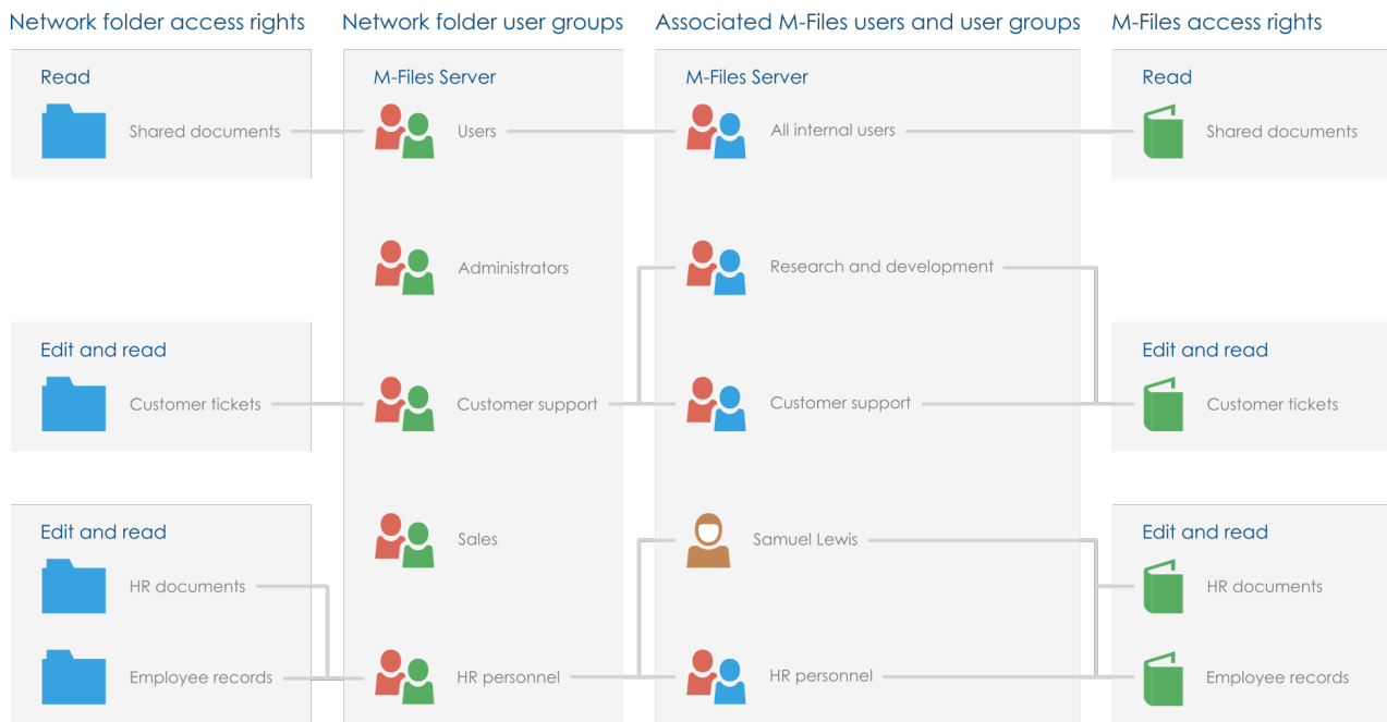
Figure 50: To refine access rights of external repository content, you must map external repository user groups with M-Files users and user groups in M-Files Admin.
