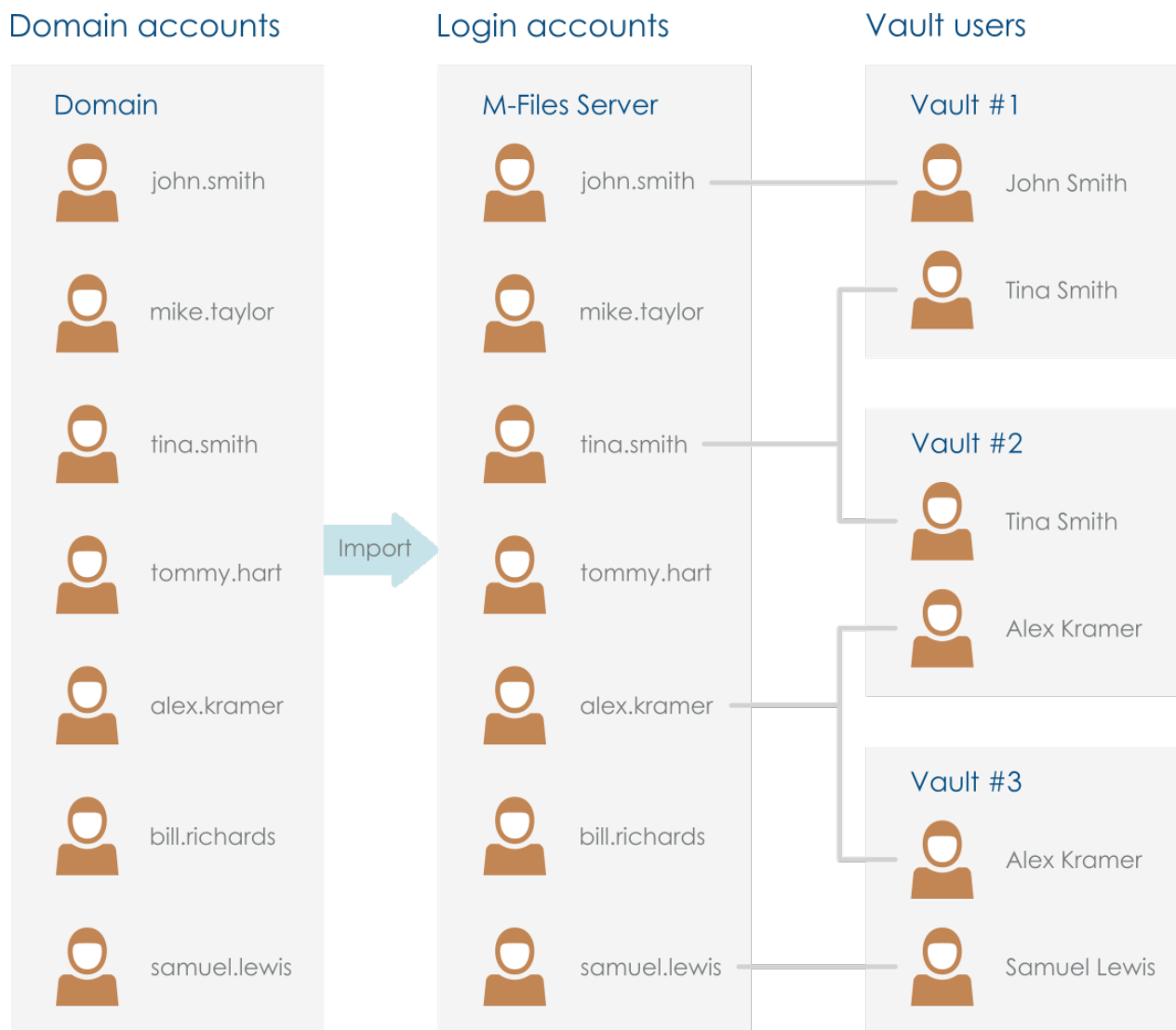
Figure 24: Login accounts are used for authenticating M-Files users to M-Files Server. They can be imported from a domain to M-Files Server. Login accounts are associated with vault-specific users.
