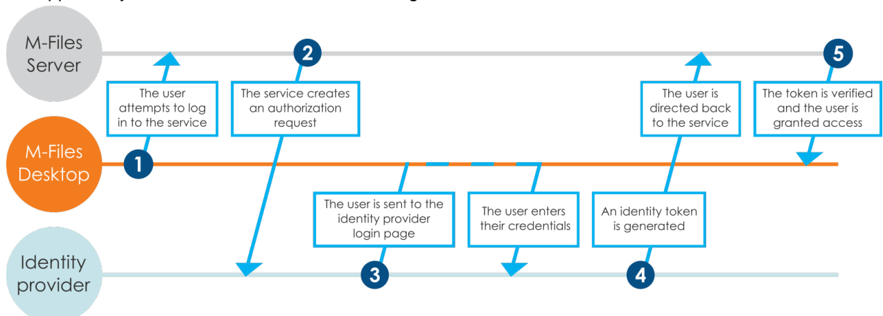
Figure 20: Authentication flow in a federated authentication system.
