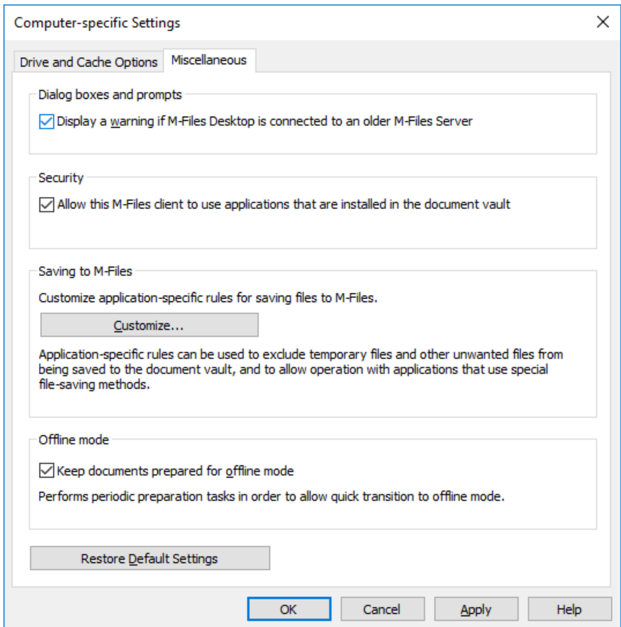
Figure 14: The Miscellaneous tab contains different computer-specific settings.
